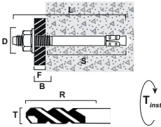
Betong
